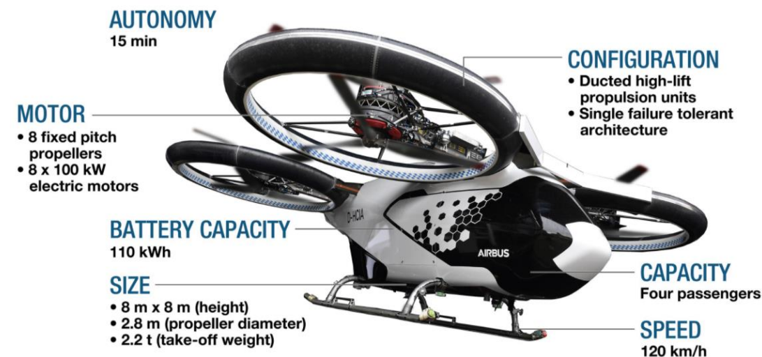
Figure 3: Example concept vehicle - Airbus eVTOL
